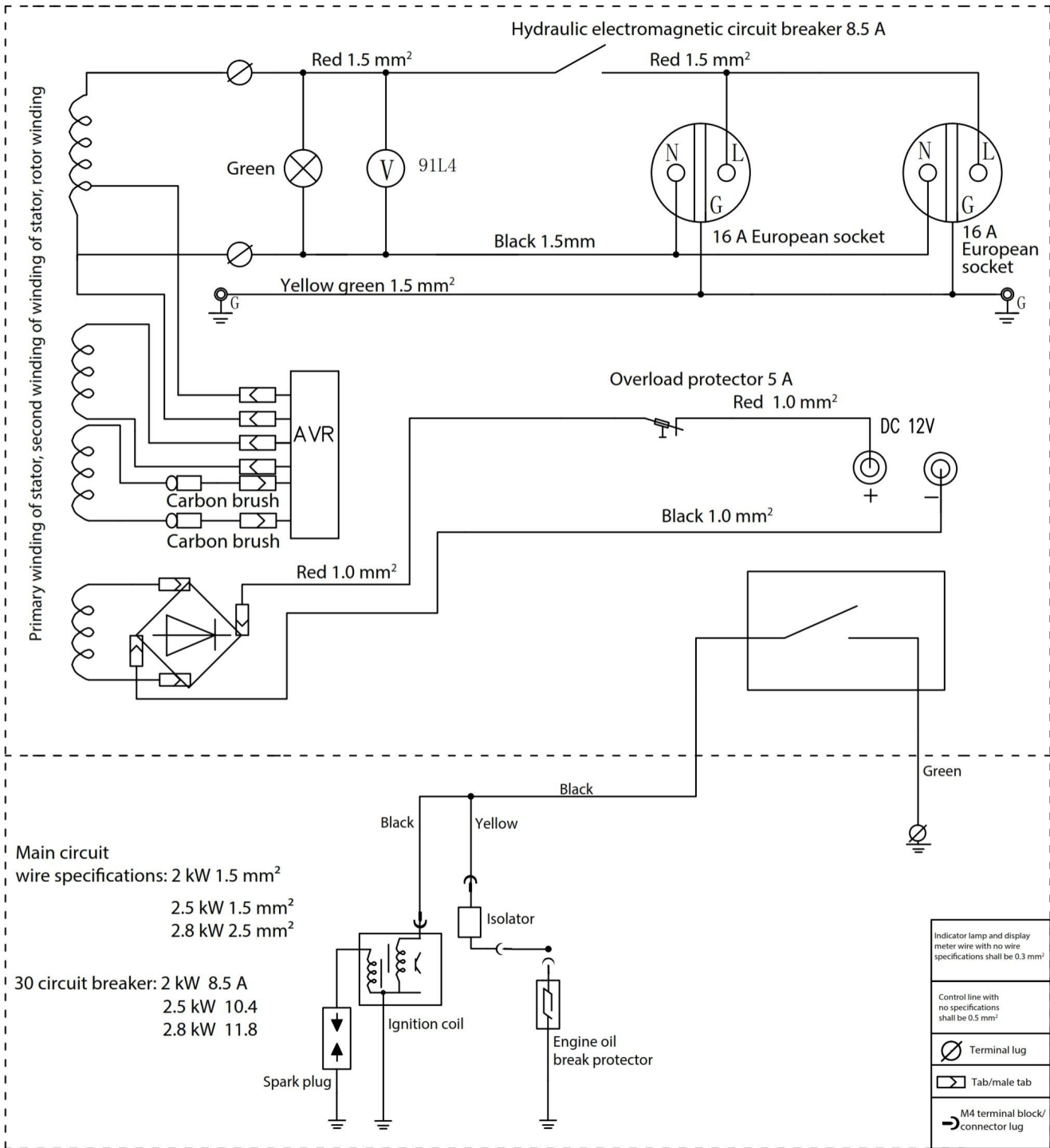
EZG3000 Electrical Schematic Diagram
